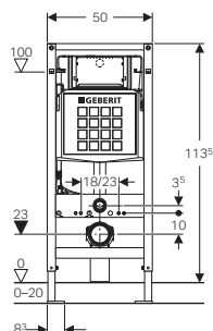
Duofix element with Sigma concealed cistern, thickness 120mm, height 1135mm
