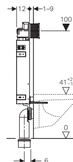
Kombifix element with Sigma concealed cistern, thickness 120mm, height 1080mm
